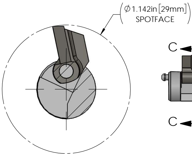
SECTION C-C SCALE 2 : 1
